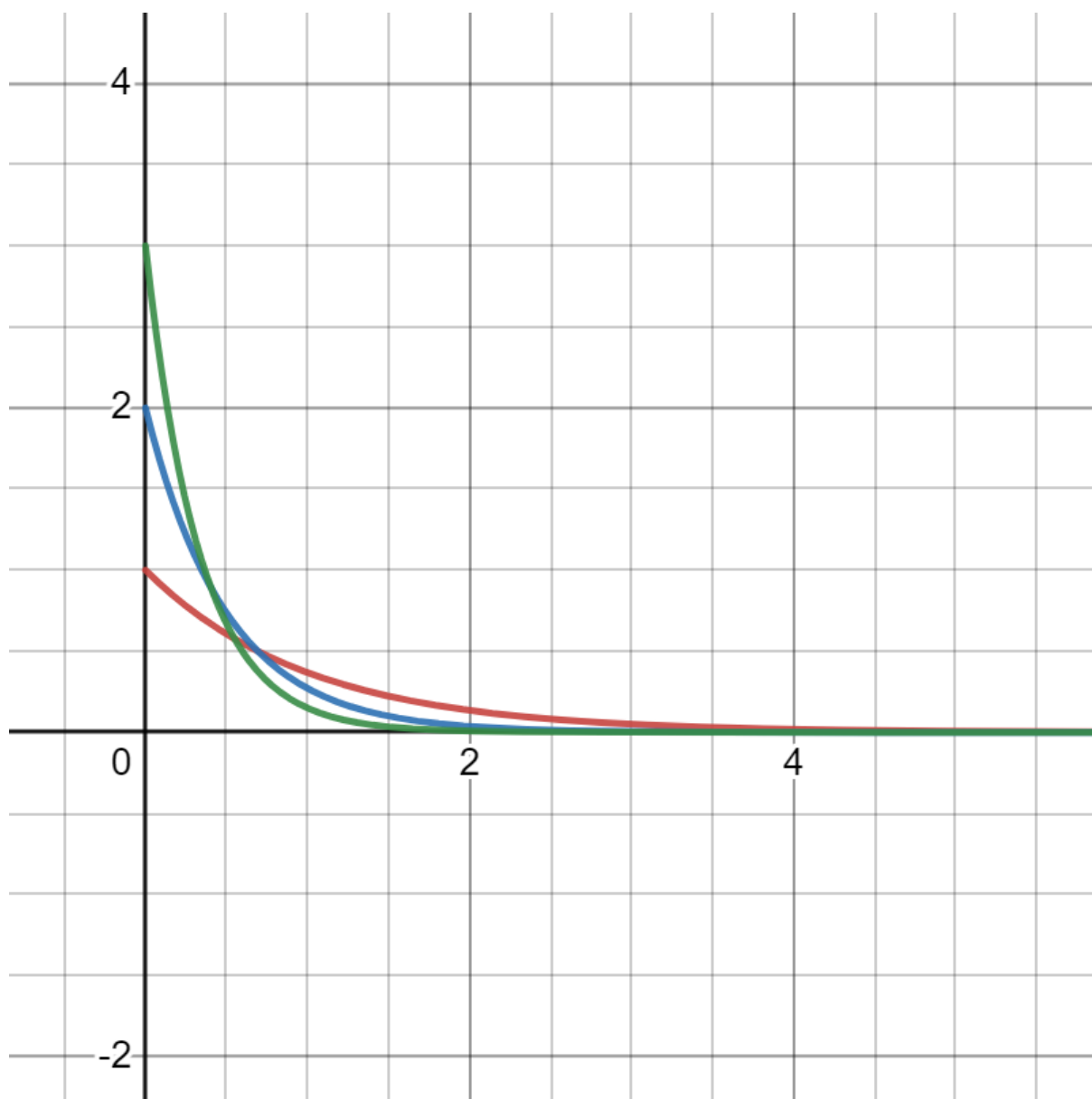
Figure 20: tightness example
