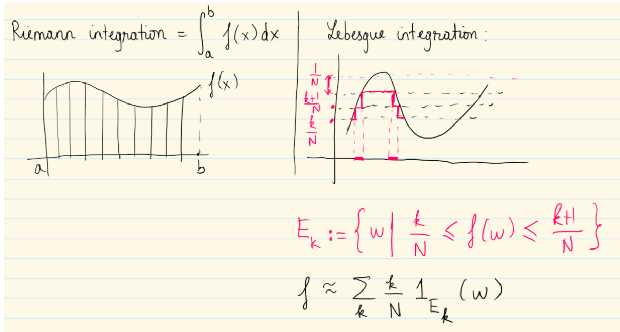
Figure 11: Riemann vs Lebesgue integral
