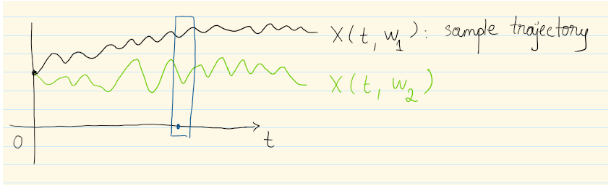
Figure 21: Stochastic Process example
