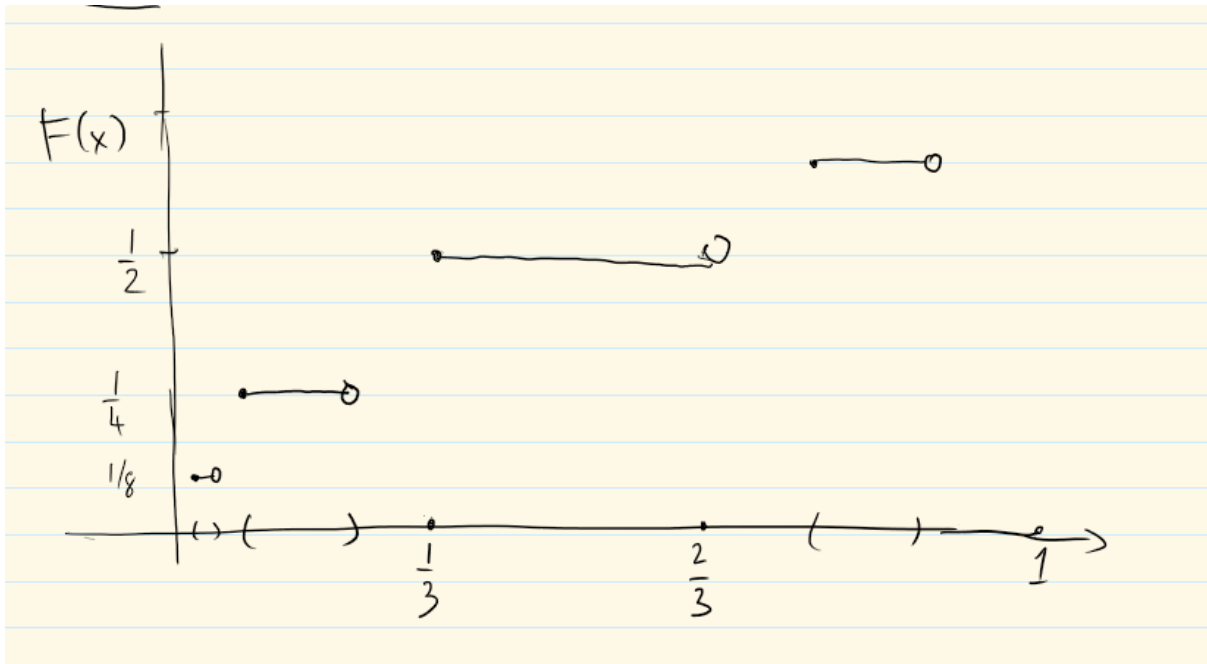
Figure 7: Devil staircase
