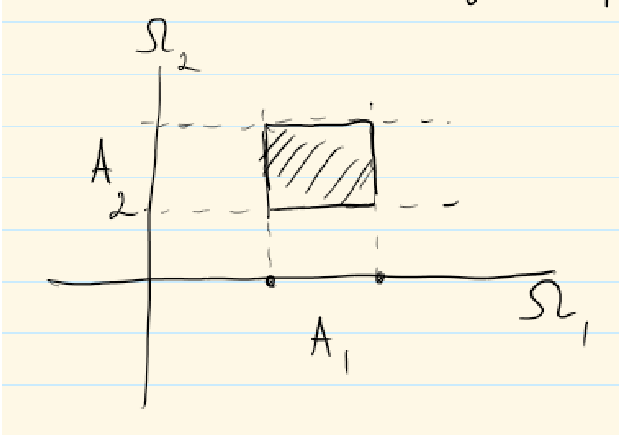
Figure 16: product measure \mu = \mu_1\mu_2
