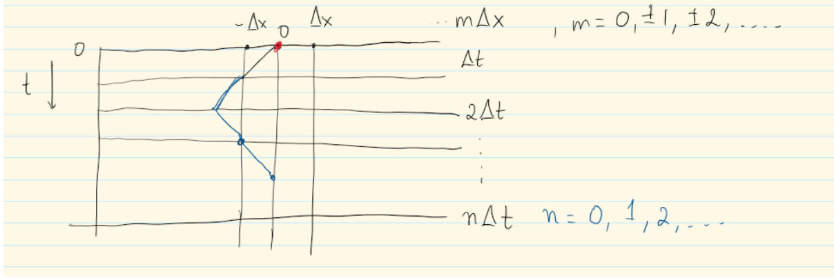
Figure 22: Random Walk
